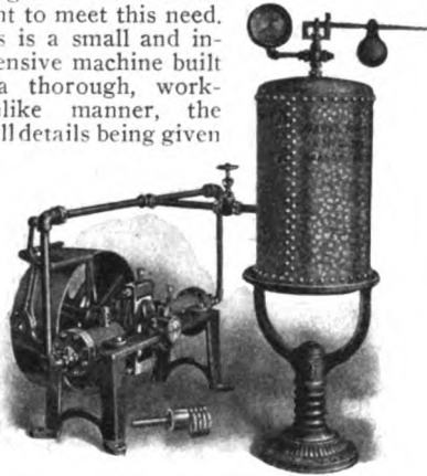
LITTLE GIANT AIR COMPRESSOR OUTFIT.
